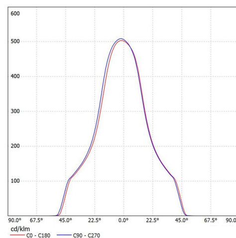
SL-04438A K:3.06cd/lm,LED:CXM-6
