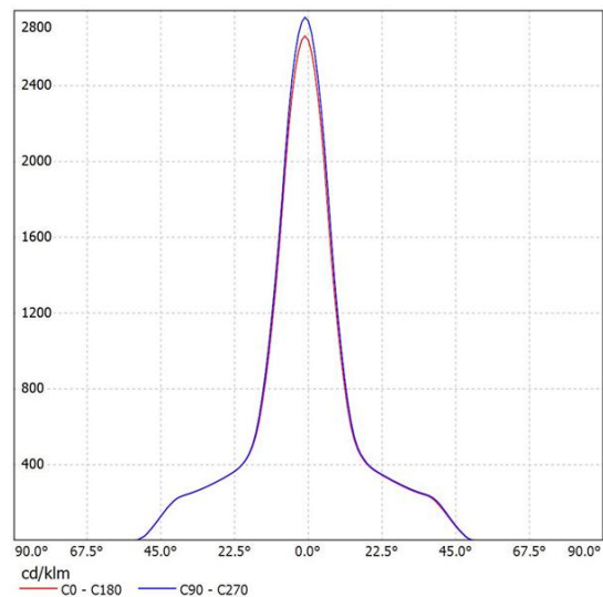
SL-04415B K:3.79cd/lm,LED:CXM-9
