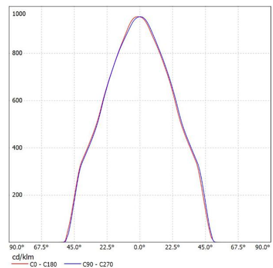
SL-04460B K:0.99cd/lm,LED:G4-10
