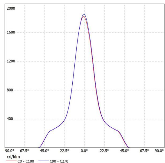
SL-04425B K:2.53cd/lm,LED:CXM-9
