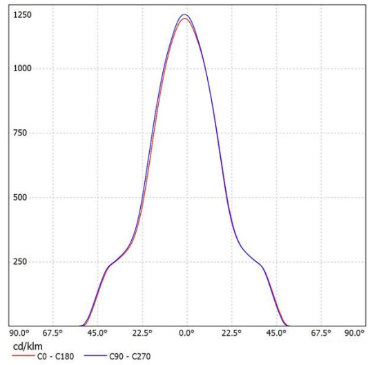
SL-04438B K:1.64cd/lm,LED:CXM-9
