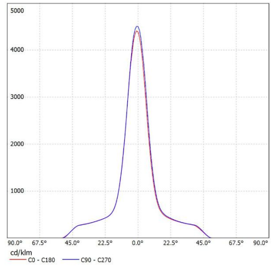
SL-04415B K:4.68cd/lm,LED:G4-10
