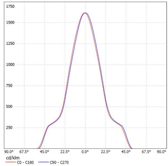
SL-04438B K:1.68cd/lm,LED:G4-10
