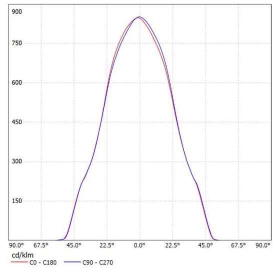
SL-04460B K:1.14cd/lm,LED:CXM-9
