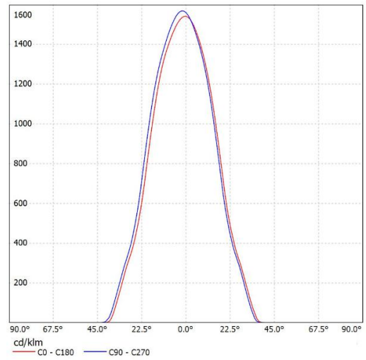
SL-05038A K:2.26cd/lm,LED:CXM-9
