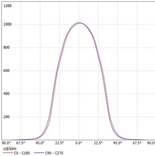
SL-05060A K:1.26cd/lm,LED:CLL02X
