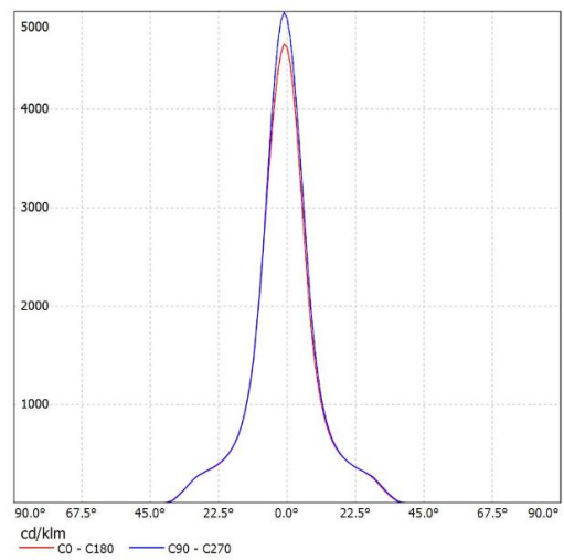
SL-05015A K:7.26cd/lm,LED:CXM-9
