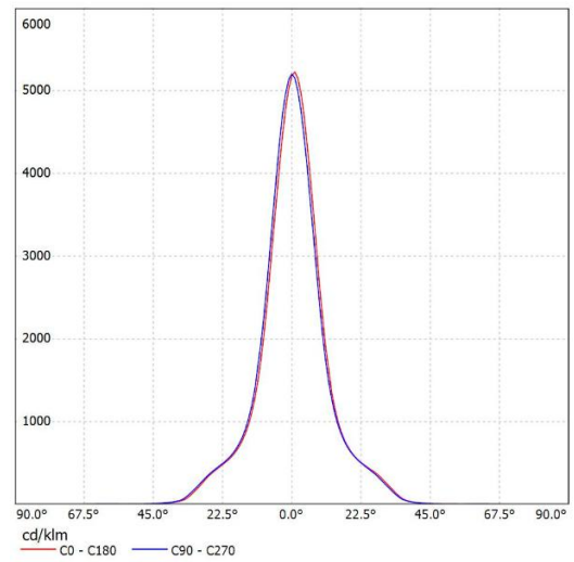
SL-05015A K:6.06cd/lm,LED:CLL02X
