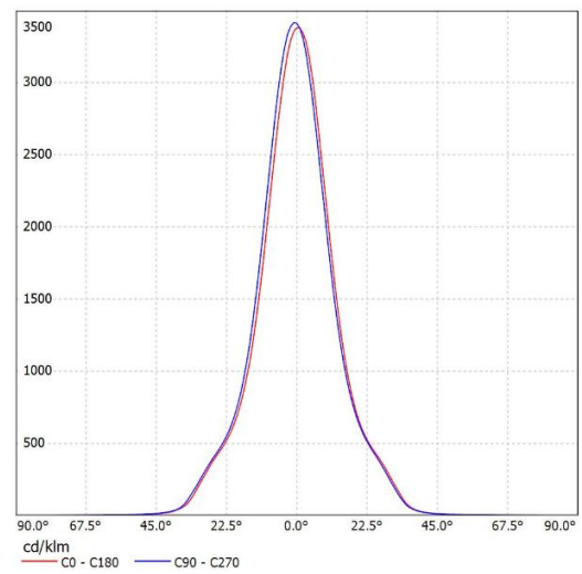
SL-05024A K:3.99cd/lm,LED:CLL02X
