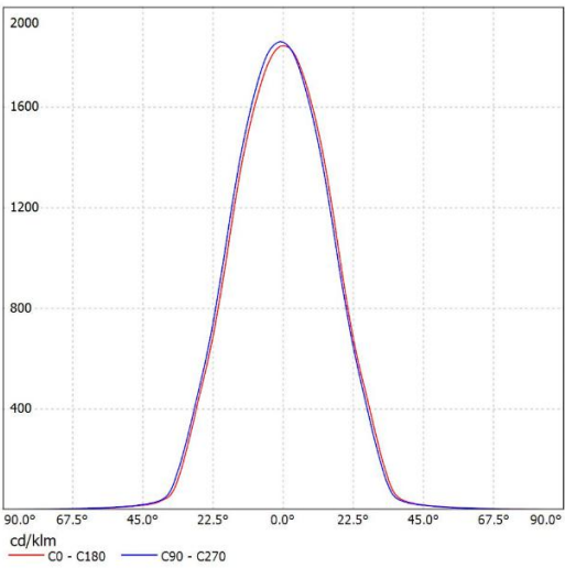
SL-05038A K:2.20cd/lm,LED:CLL02X
