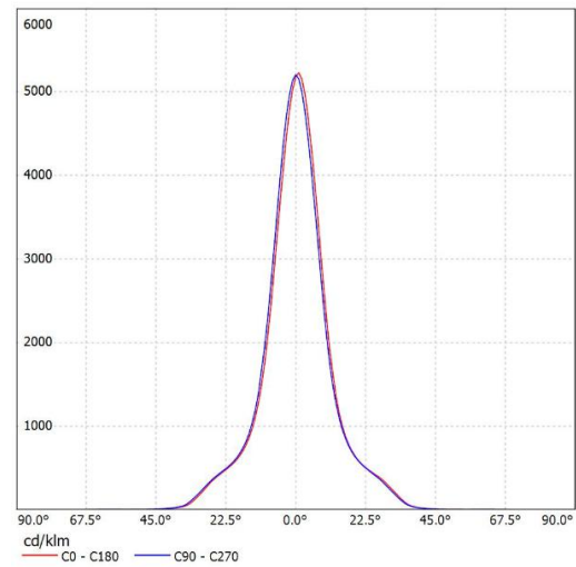
SL-05015D K:6.06cd/lm,LED:CLL02X
