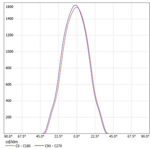
SL-05038D K:2.26cd/lm,LED:CXM-9
