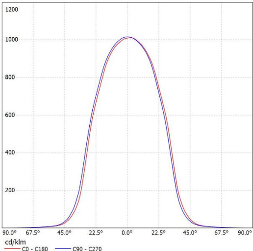
SL-05060D K:1.26cd/lm,LED:CLL02X
