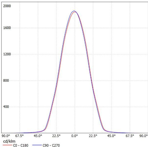
SL-05038D K:2.20cd/lm,LED:CLL02X
