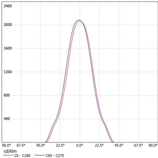
SL-05038D K:2.64cd/lm,LED:1507
