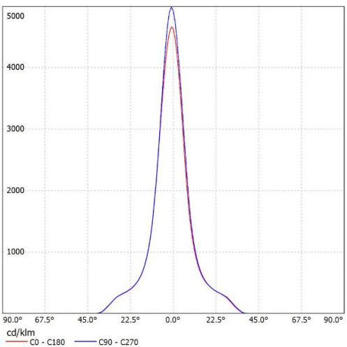
SL-05015D K:7.26cd/lm,LED:CXM-9
