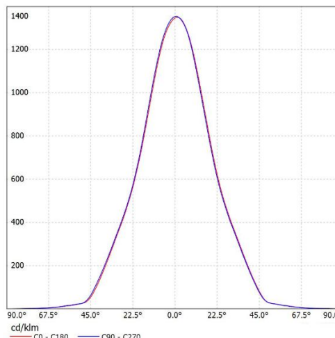
SL-03540B K:1.57cd/lm,LED:V10 Gen7
