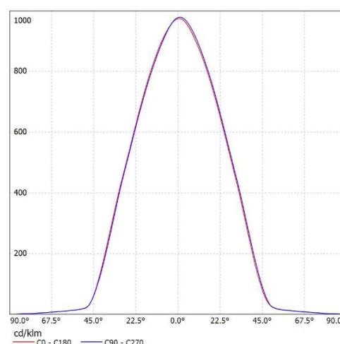
SL-03540B K:1.13cd/lm,LED:V10 Gen7
